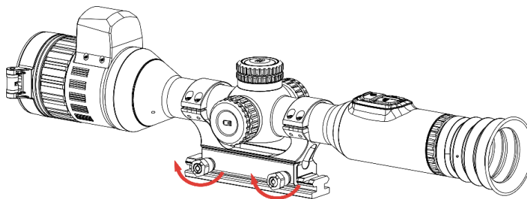
Figure 2-9 Serrage des vis
